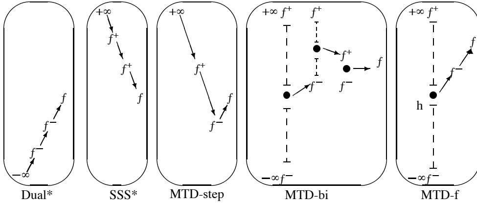
Figure 9: MT-based algorithms.
