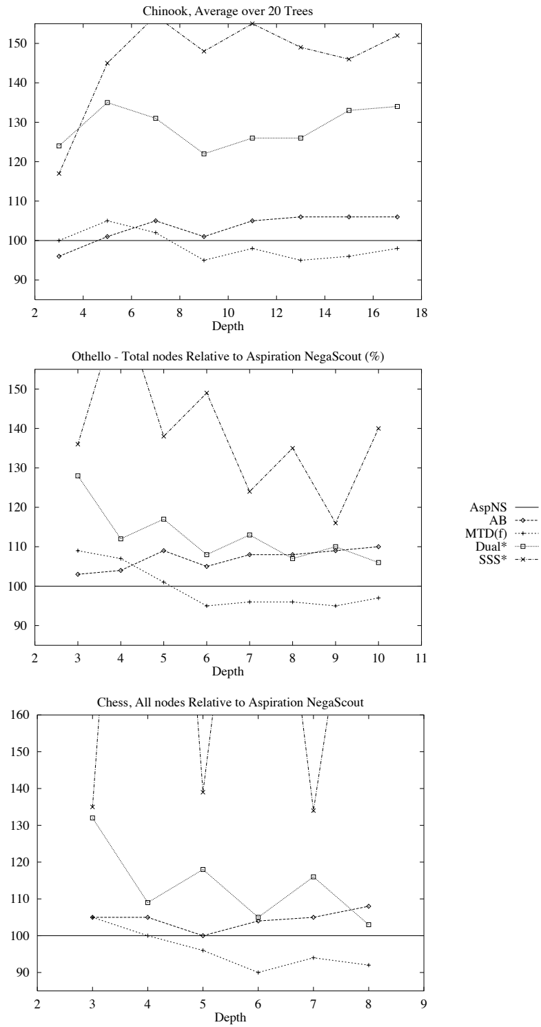
Figure 12: Total node count
