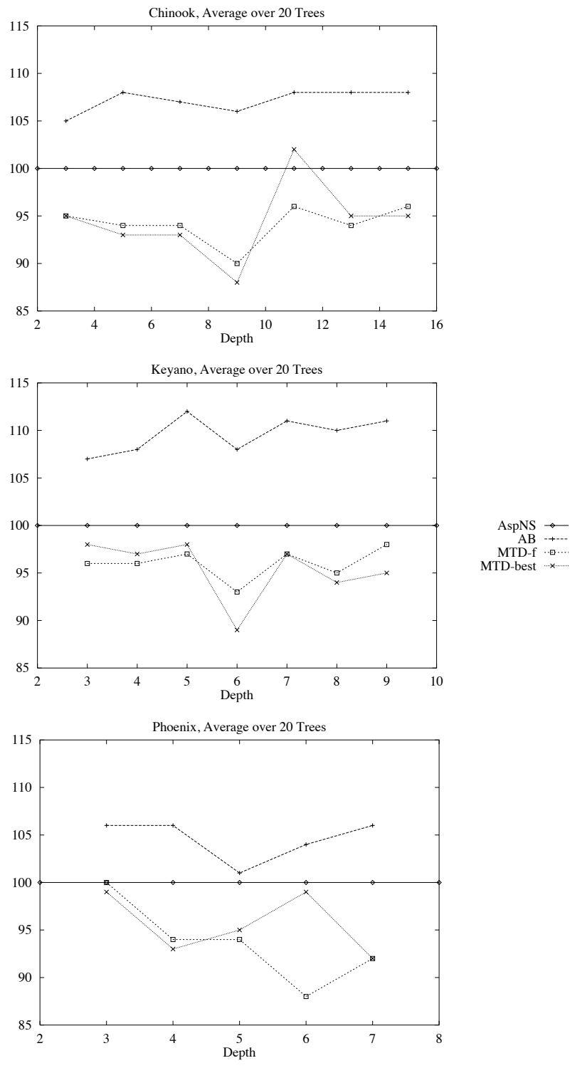
Figure 14: Leaf node count MTD-best
